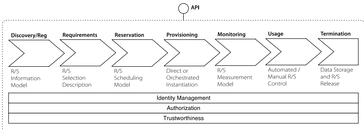
Figure 15: Experiment Lifecycle
